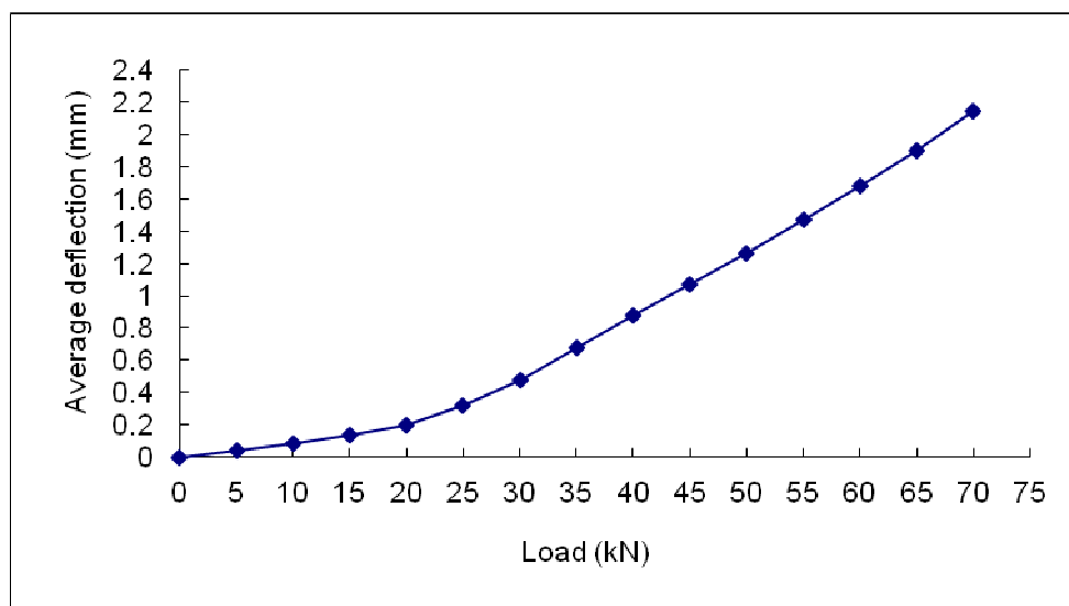
Fig.2: Average Deflection-Load Graph of Sample2
