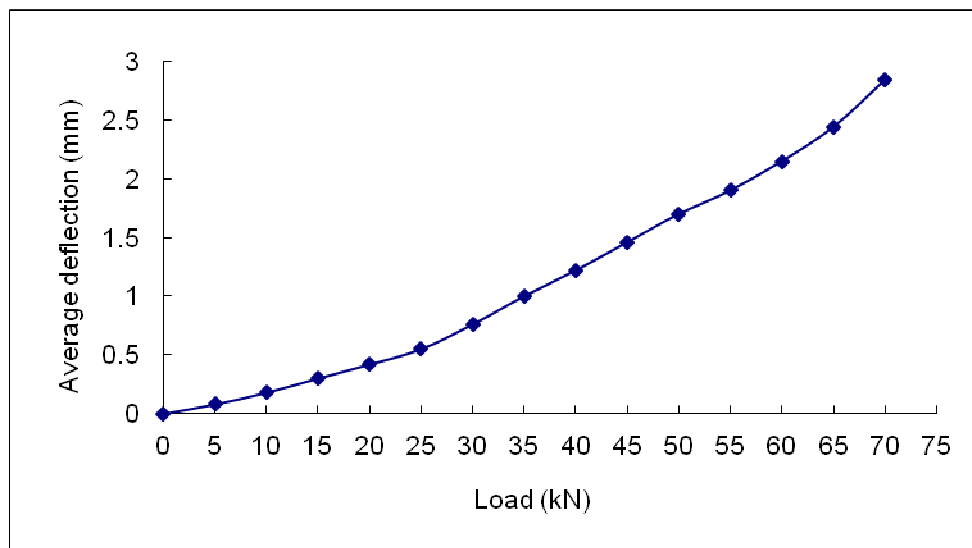
Fig.1: Average Deflection-Load Graph of Sample1
